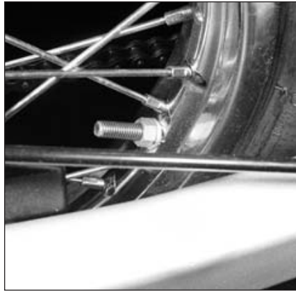
5.7 Tighten the locknut on the rim lock to the specified torque
