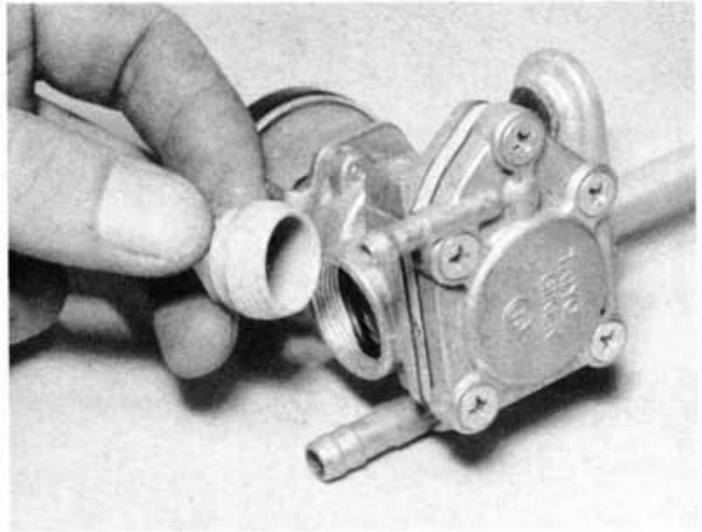
3.4 Sediment bowl is located on the underside of the tap body
