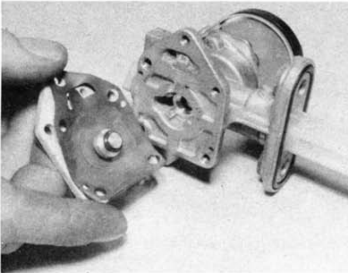
3.3b Fuel valve is on inner face of the diaphragm assembly
