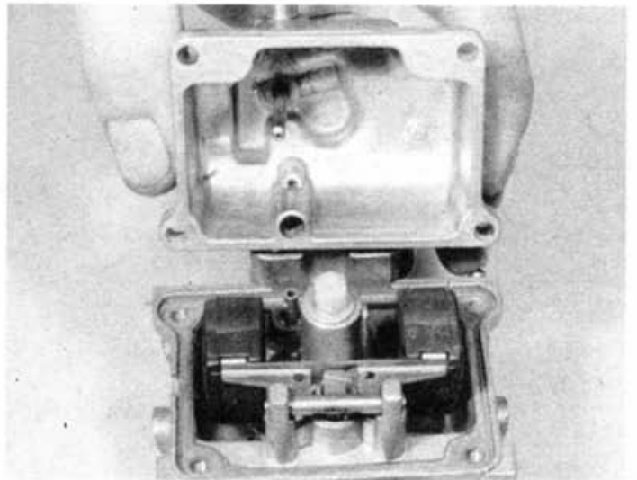
6.1 Remove the four screws and lift away the float bowl
