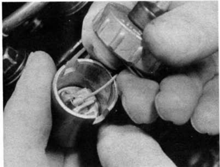
5.4 Compress the return spring, then disengage the inner cable
