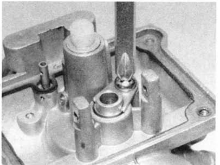
6.2b Release the single screw and retainer ...
