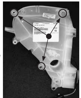
Figure 1.2 - Back view of brake side cabinet
