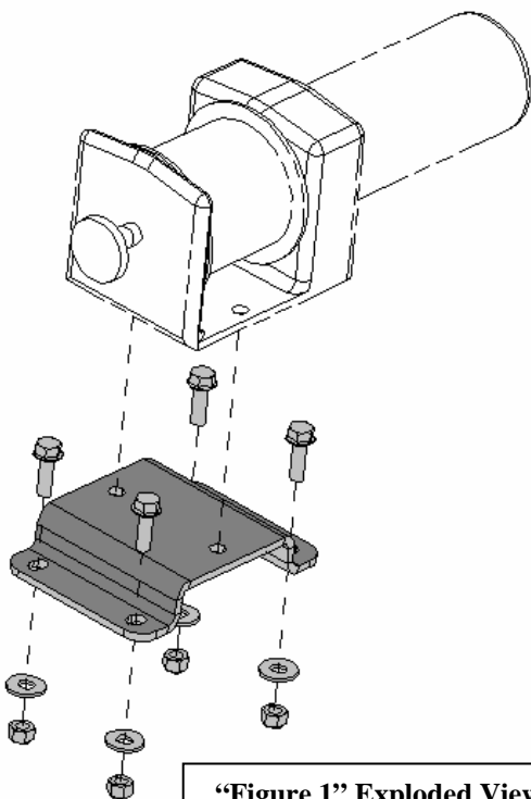
"Figure 1" Exploded View
