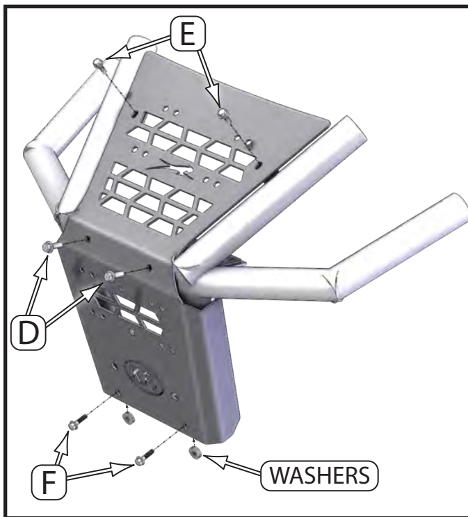
"Figure 4" Grill Plate Install
