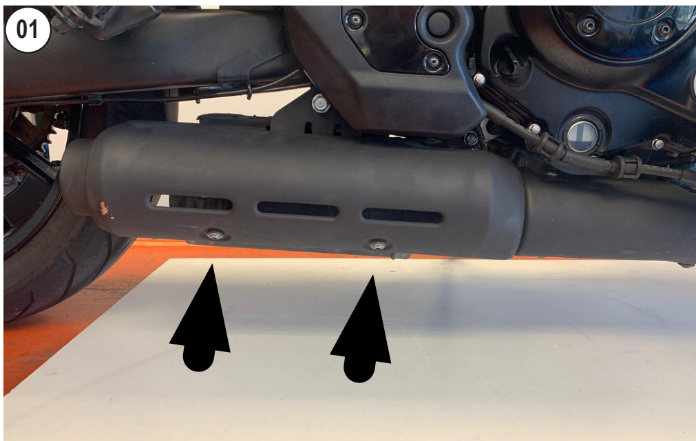
UNSCREW AND REMOVE THE STOCK HEAT SHIELD
