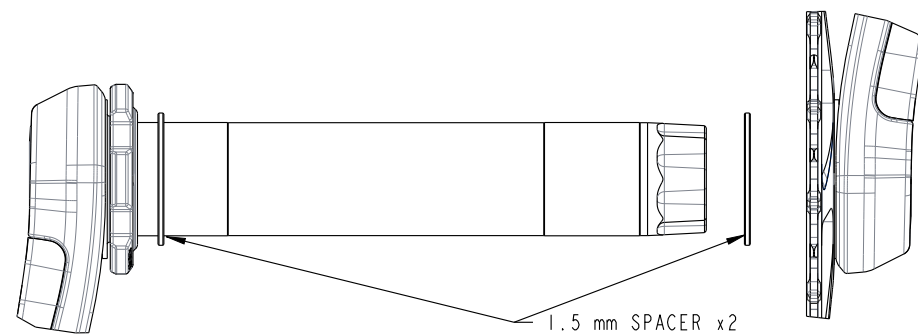
RF169 SPINDLE
