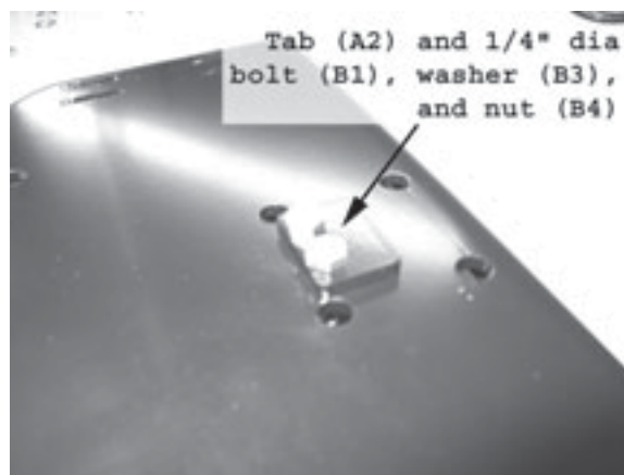
Figure1 Attach Tab to Plow Mount
