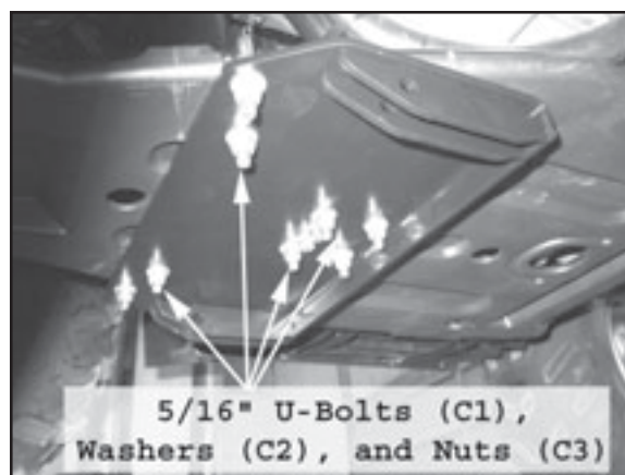
Figure3 Attach Plow Mount to Vehicle
