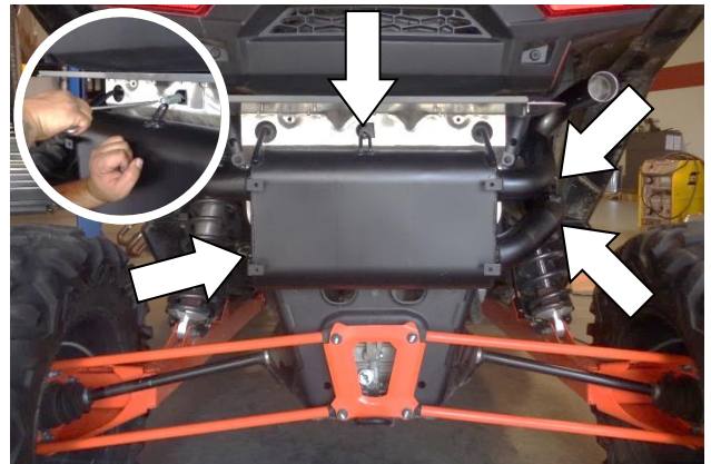
11. Use a spring puller to connect the four muffler mount springs to the new muffler.
