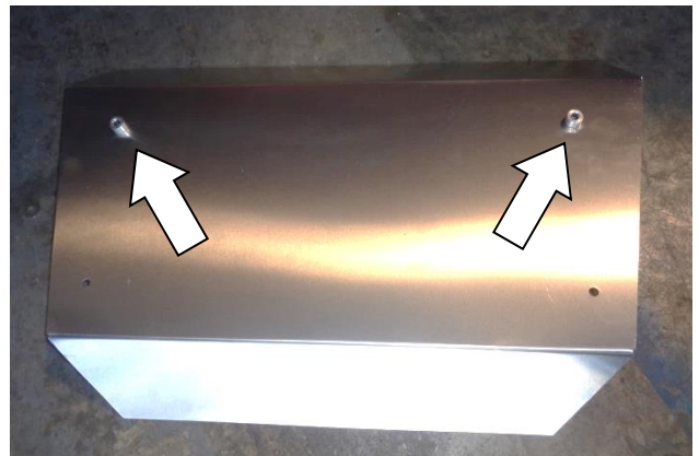
12. Place the heat shield backer (2) on a bench or other flat surface. Place spacers (7) over the top two holes.
