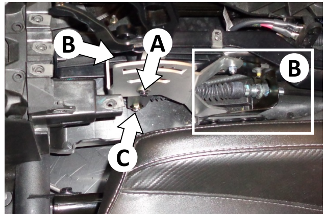
37. Tighten the shifter hardware in the following order: pivot screw (A); shifter gate and cable support screws (5 places; B); and cable end nut (C).
