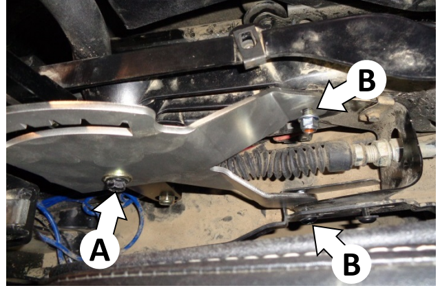
35. Hand-start (do not tighten) the pivot screw, nut and washers (A), and the front cable support screws and nuts (5) (B).
