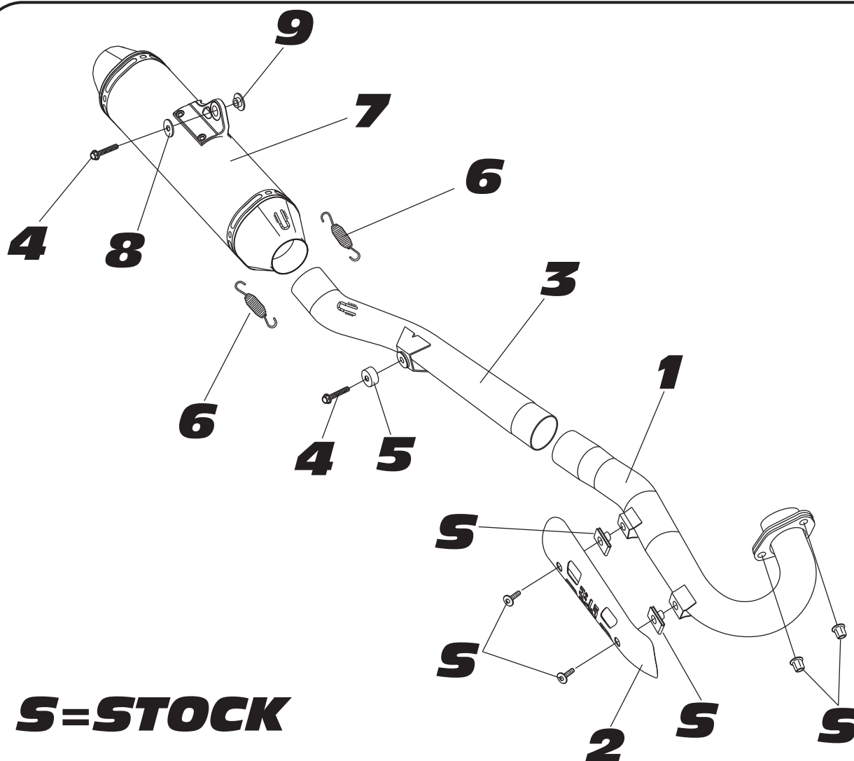
Parts Diagram
